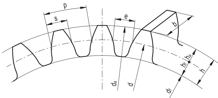
Fig.1: a tooth profile
