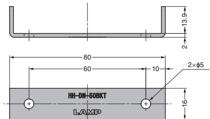
HH-DN-50BKT
