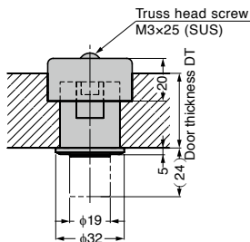
[Door Thickness 24~23 mm]
