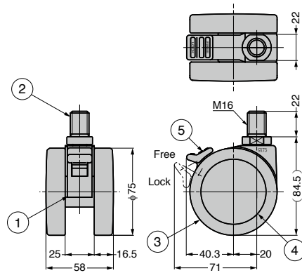
Drawing above shows the model with brake.
