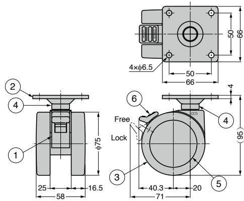
Drawing above shows the model with brake.
