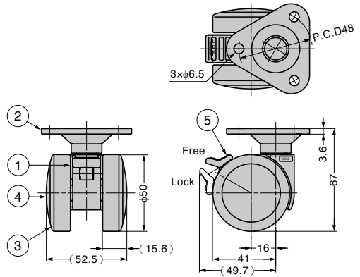
Drawing above shows the model with brake.
