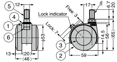
Drawing above shows the model with brake.
