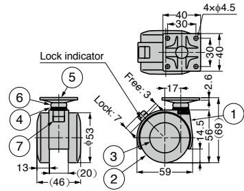
Drawing above shows the model with brake.
