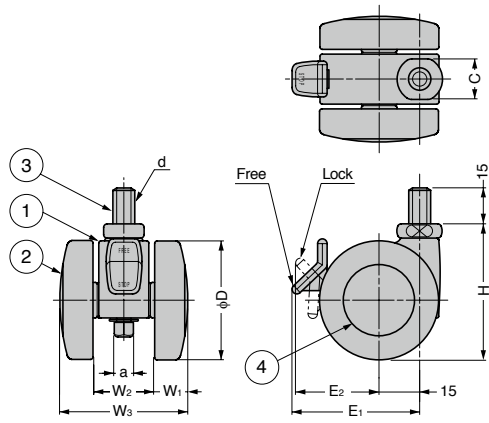
Drawing above shows the model with brake.
