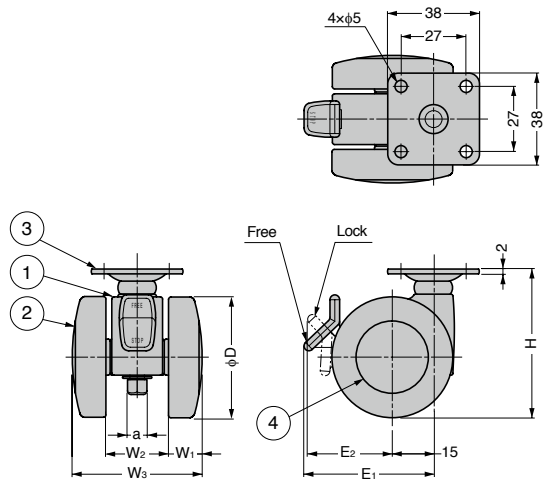
Drawing above shows the model with brake.
