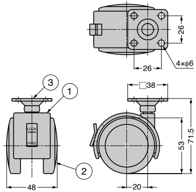
Drawing above shows the model with brake.
