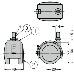
Drawing above shows the model with brake.
