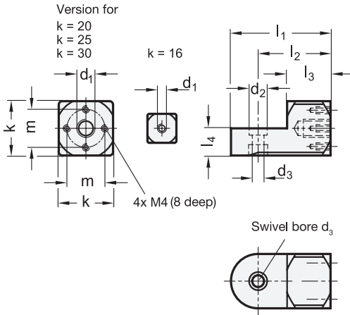
Mounting clamp joint with clamping kit GN 511.1, type K
