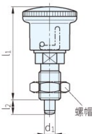
銷子外伸鎖固
